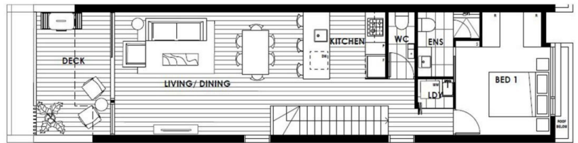
FIRST FLOOR
